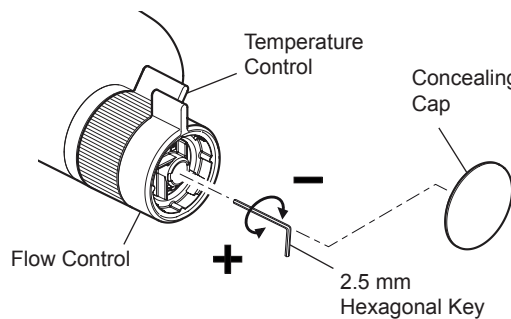
Dual Control
