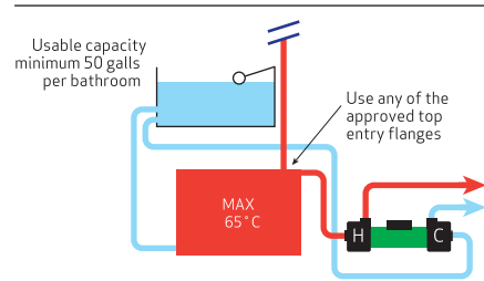
Figure 24: Horizontal cylinders
