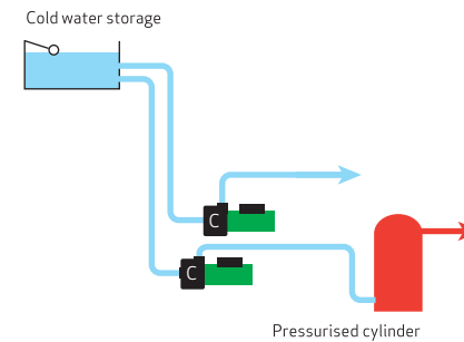
Figure 12: Pressurised cylinder or Combination boiler system
