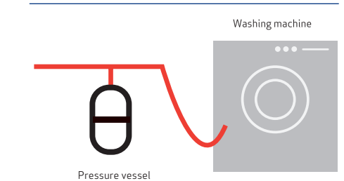
Figure 28: Water hammer protection
