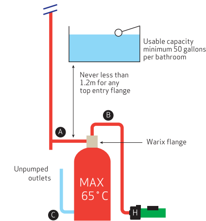
Figure 26: Approved flanges
