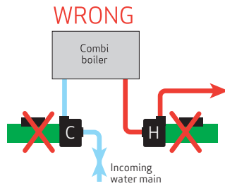
Figure 23: Combi boilers
