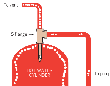
Figure 25: S flange
