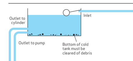
Figure 1: Tank inlet and outlet position
