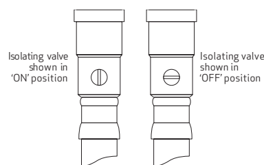
Figure 4: Isolating valves
