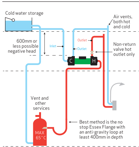
Figure 22: Anti-gravity loop (AGL)
