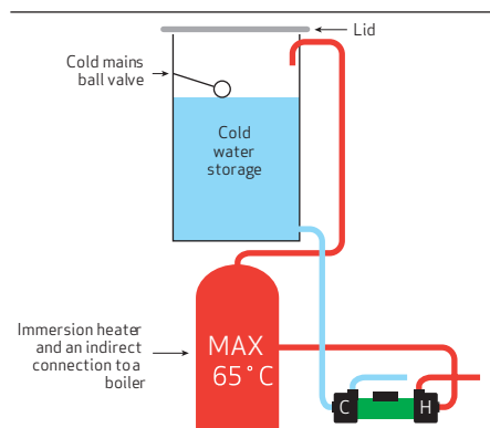
Figure 18: Pre-plumbed direct or indirect combination units
