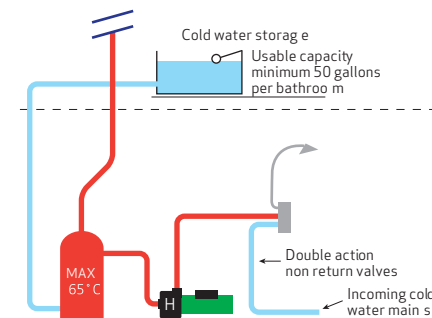
Figure 13: Tank fed (hot) with mains cold
