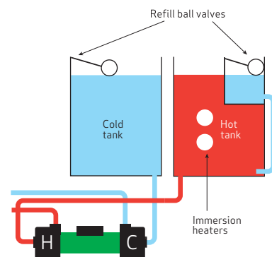
Figure 19: Elson (type) tanks
