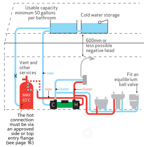
Figure 8: Whole house system Either side of these pumps can be used for hot or cold water.
