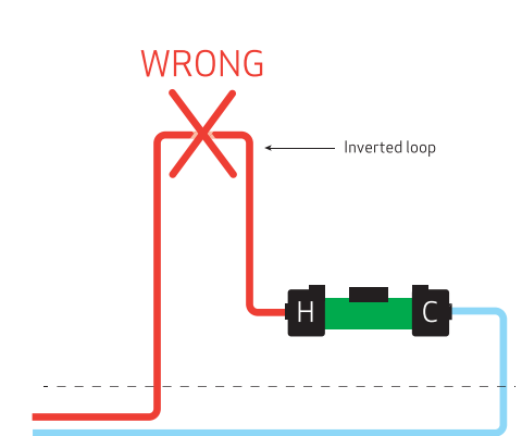
Figure 27: Inverted loops
