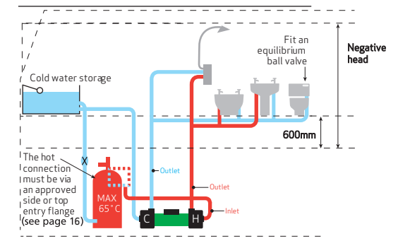
Figure 9: Negative head
