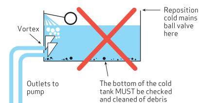
Figure 16: Aeration
